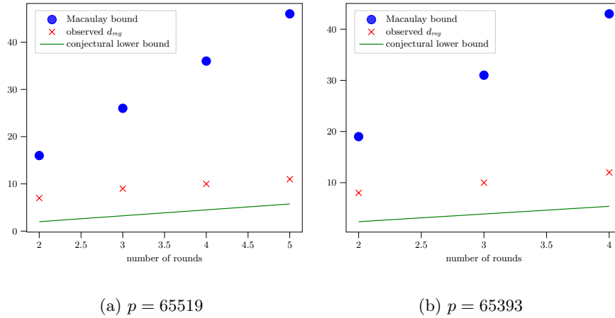
Fig. 3: evolution of the degree of regularity
