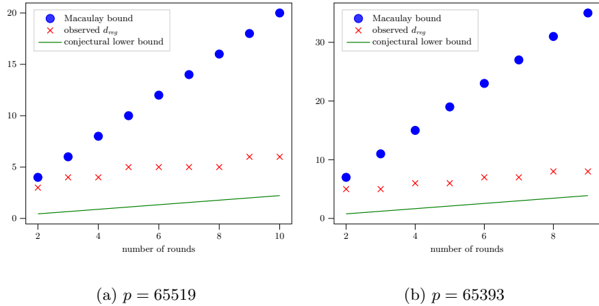
Fig. 4: evolution of the degree of regularity when the Legendre symbols are known
