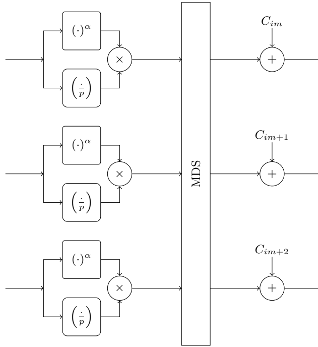
Fig. 2: one round of Grendel with m = 3
