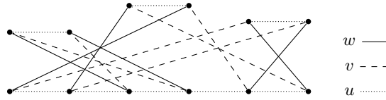
Fig. 6: Non-trivial example of a set with 12 points evenly covered by three slopes. Horizontal points lie on the same y-coordinate, and vertical points on the same x-coordinate. Since there are six points on a line with slope u , the natural graph is not regular.
